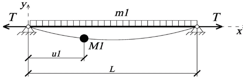
Figure 6. Dynamic model of a «damper on the thread» oscillation.
